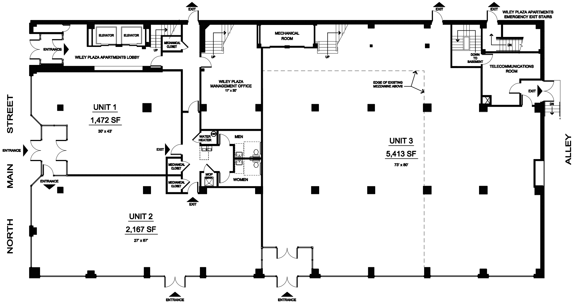
WILEY PLAZA COMMERCIAL FIRST FLOOR PLAN (CONCEPT 2) PUTNAM ARCHITECTURE, L.L.C.
